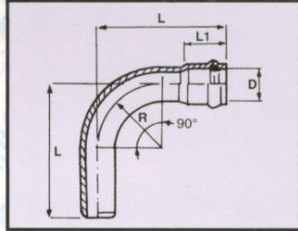
Long Bend Rubber Ring Socket / Spigot 90°
