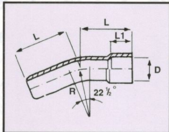
Long Bend Solvent Cement Socket/Spigot 22,5°
