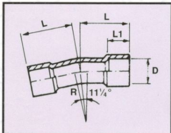
Long Bend All Solvent Cement Socket 11,25°
